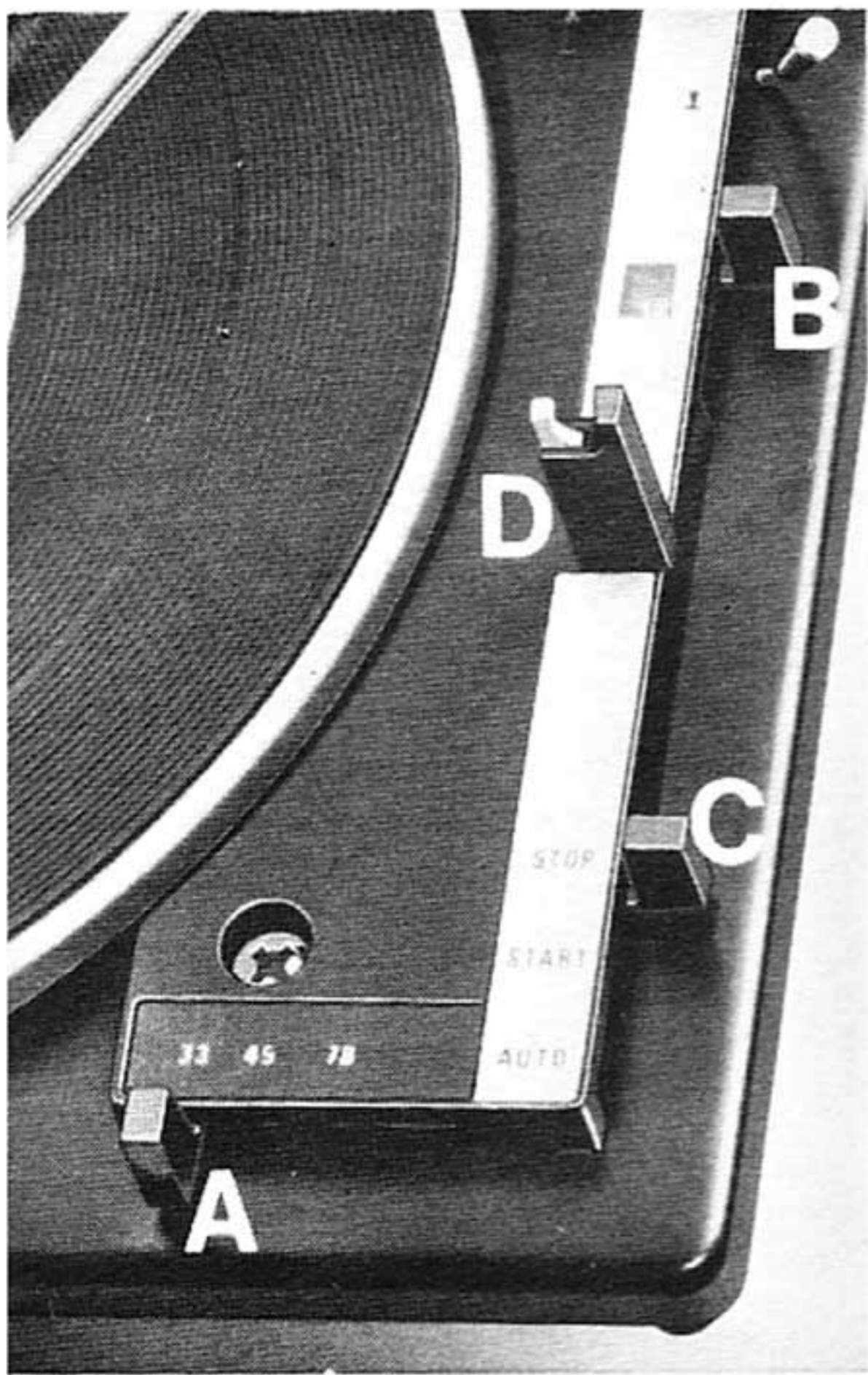
1 CONTROL PANEL WITH AUTOMATIC PICK-UP LOCK
